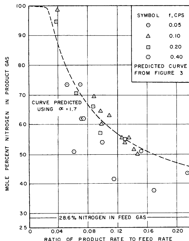
Fig. 5. Product gas compositions for various flow conditions at 20 lb./sq.in. gauge feed gas pressure and at 24°C. (42-60 mesh particles of Type 5A Molecular Sieve).
