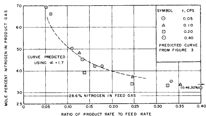
Fig. 4. Product gas compositions for various flow conditions at 10 lb./sq.in. gauge feed gas pressure and 24°C. (42-60 mesh particles of Type 5A Molecular Sieve).
